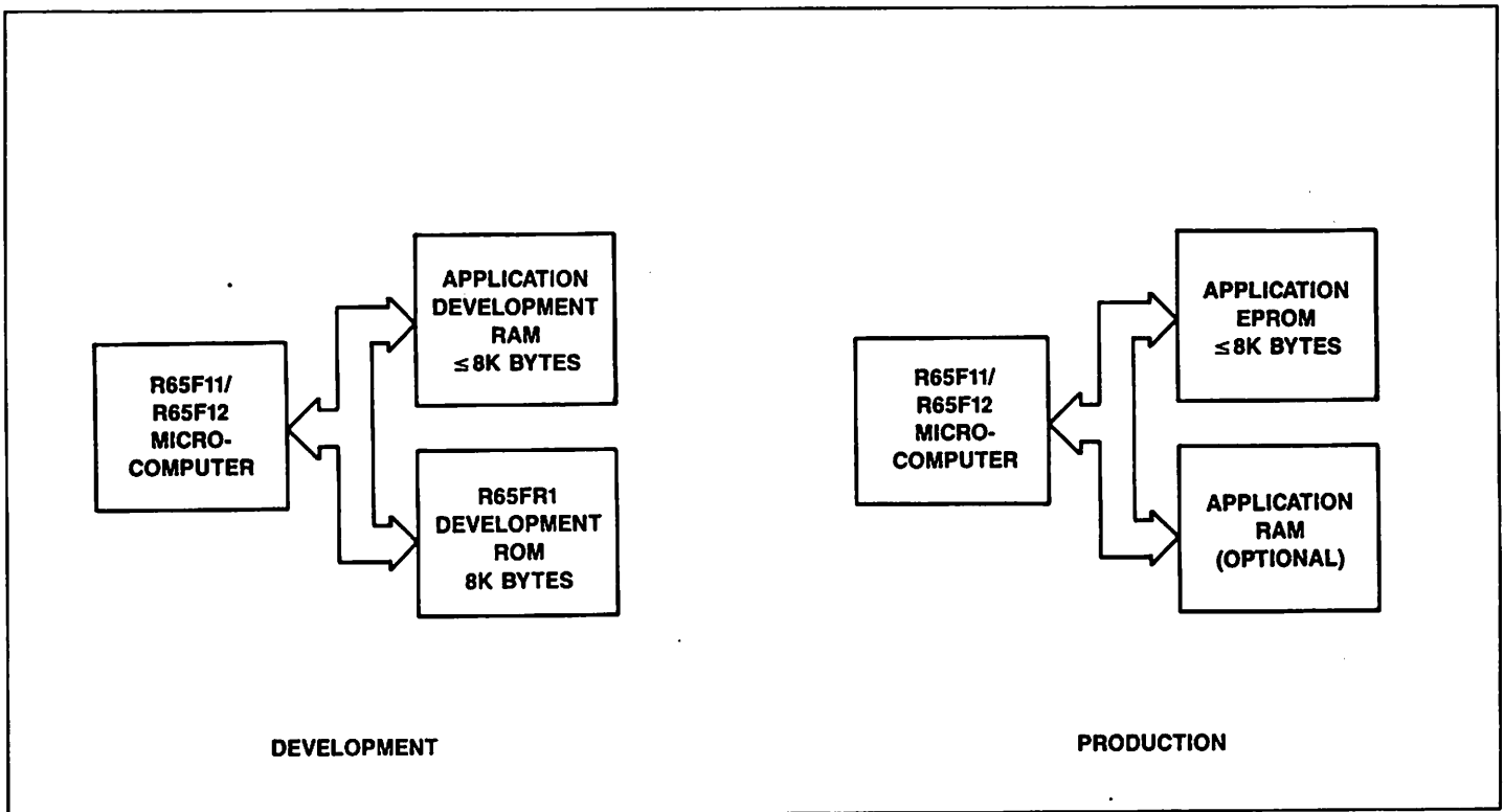
Figure 1. R65FR1 Configuration 1 Block Diagram
