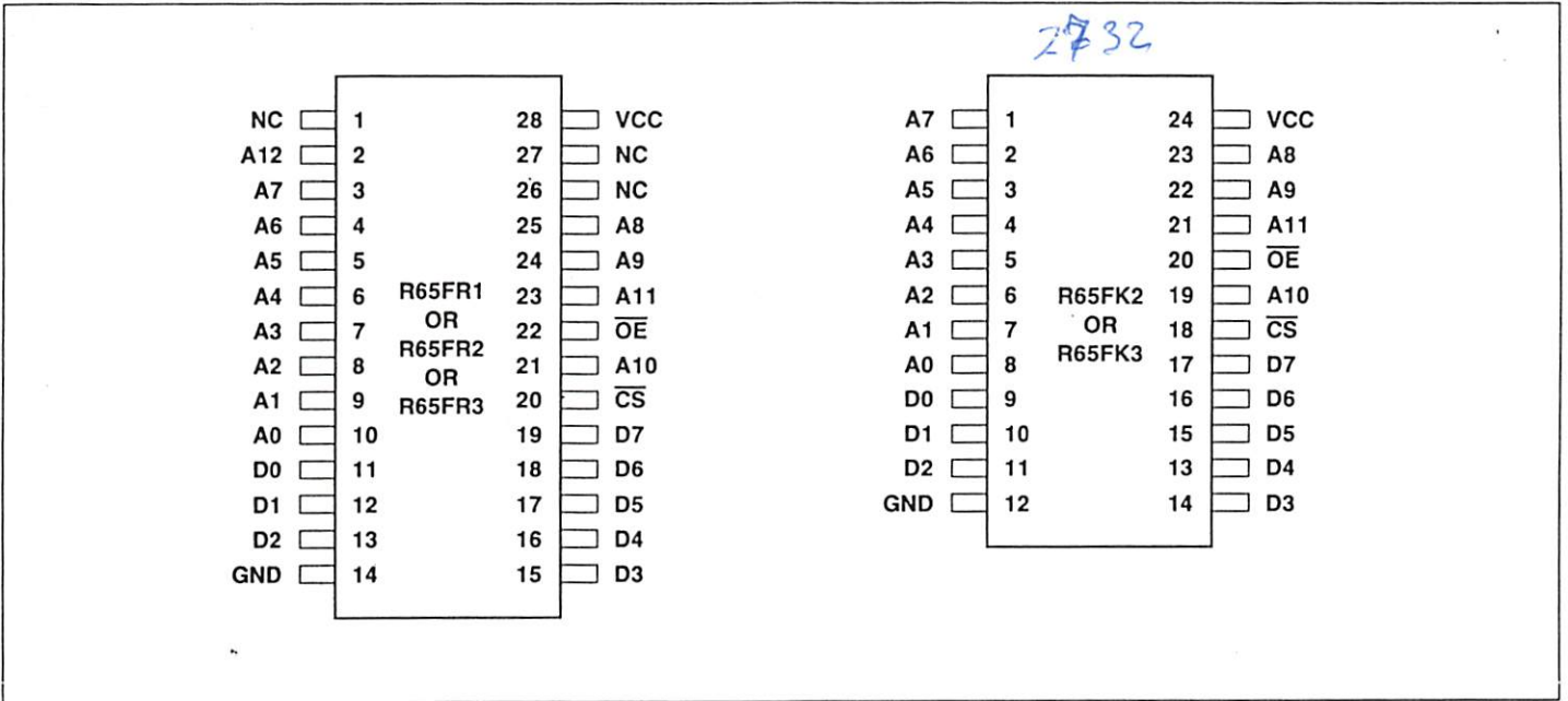
RSC-FORTH ROM Pin Assignments
