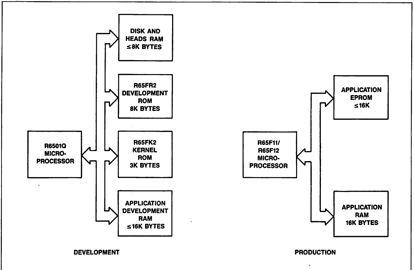
Figure 2. R65FR2 and R65FK2 Configuration 2 Block Diagrams
