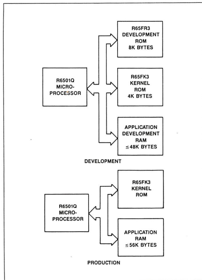
Figure 4. R65FR3 and R65FK3 Configuration 3 Block Diagrams
